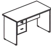
OFB 1260 1200W X 600D X 750H
